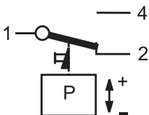
Manual reset high pressure contact function
