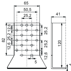
Univ. mounting bracket 0 714 147 (incl. screws)
