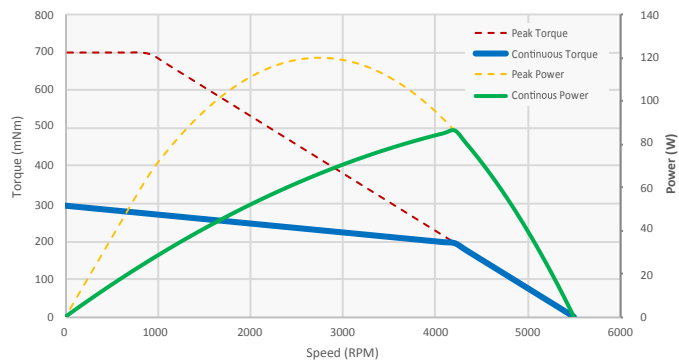
RPX52-600 Performance
