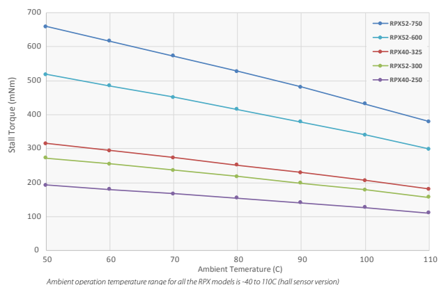
RPX Series Stall Torque at Elevated Ambient Temperatures
