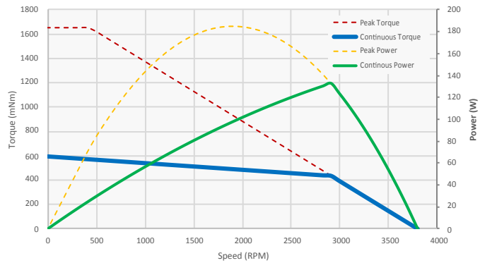
RPX52-750 Performance
